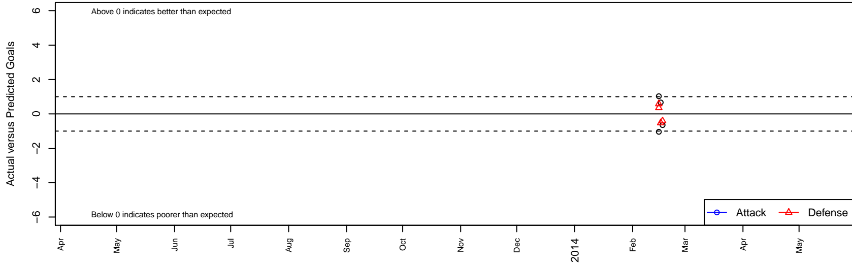
FC Dallas El Paso 00 Morin B99 Dots are actual minus expected GF (blue circles) and GA (red triangles). Blue line is smoothed change in attack strength. Red is smoothed change in defense strength.
